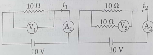
Circuit 2
